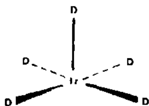
Fig. 1. Structure of \text{IrD}_5^{4-} .
