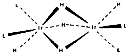
Fig. 3. Representation of the inner \text{OsH}_4\text{P}_3 core of \text{OsH}_4(\text{PMe}_2\text{Ph})_3 .
