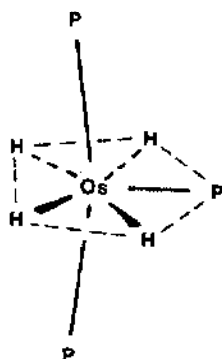
Fig. 3. Representation of the inner \text{OsH}_4\text{P}_3 core of \text{OsH}_4(\text{PMe}_2\text{Ph})_3 .
